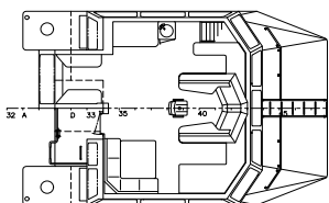
Wheelhousedeck
