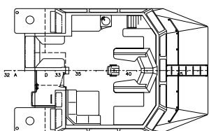
Wheelhousedeck
