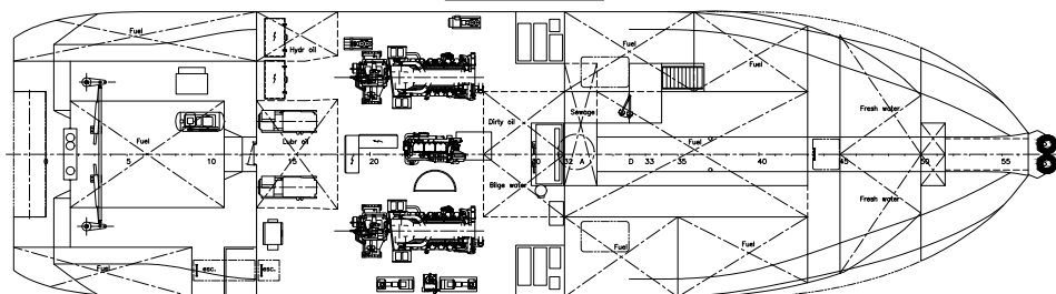
Below maindeck
