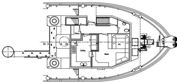
Forecastledeck
