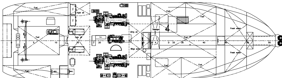
Below maindeck
